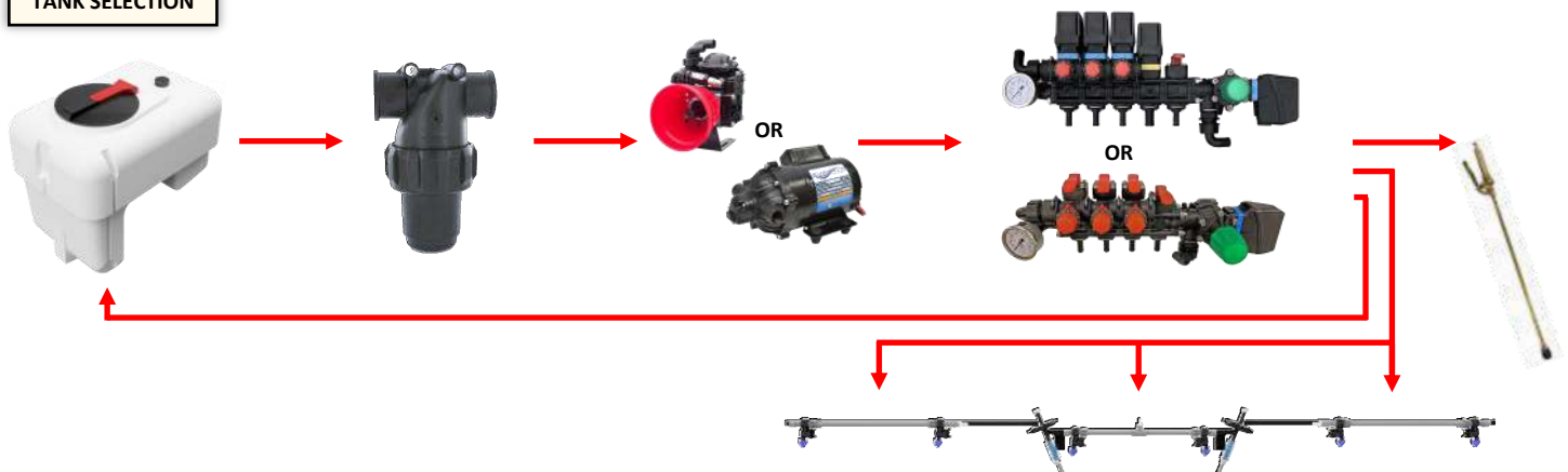
TANK SELECTION
